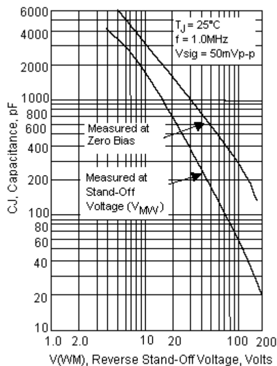
Figure 4 Typical junction Capacitance Uni-Directional
