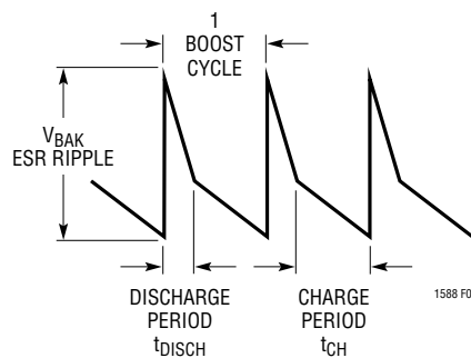
Figure 3. V_{BAK} Ripple
