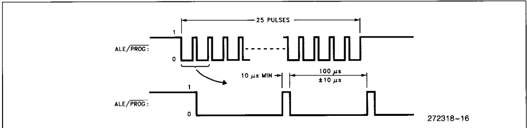
Figure 9. PROG Waveforms
