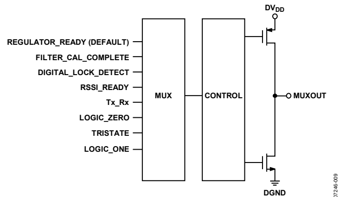
Figure 36. MUXOUT Circuit
