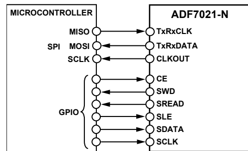
Figure 61. ADF7021-N (SPI Mode) to Microcontroller Interface
