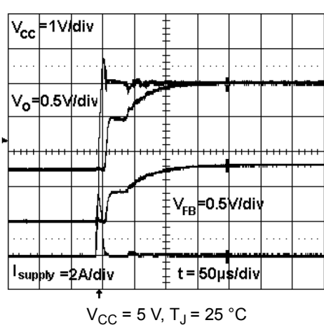
Figure 21. Startup transient
