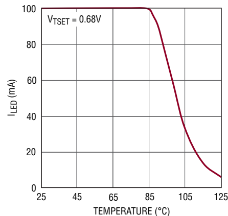
TSET LED Current Derating
