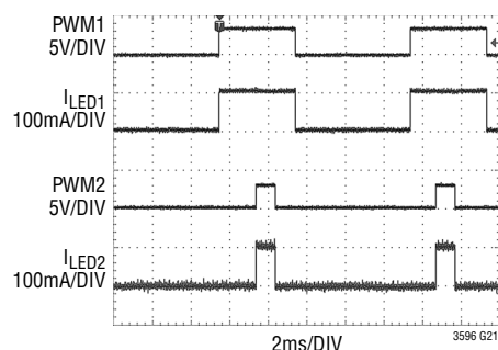
PWM Dimming Waveforms (Overlapping PWM Signals)
