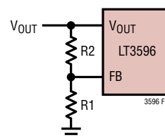
Figure 11. Programming Maximum V_{OUT}
