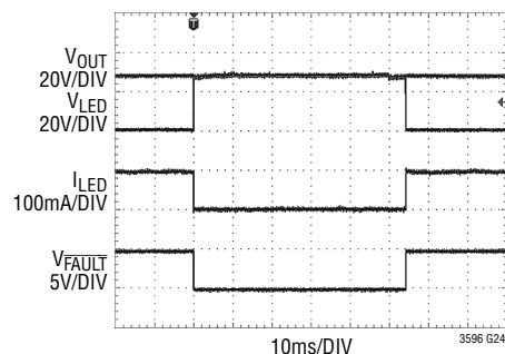
LED Short to V_{OUT} Waveforms
