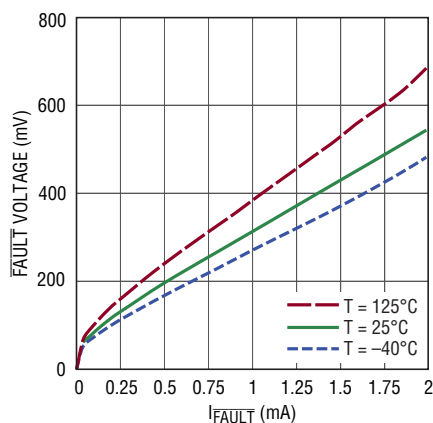
V_{FAULT} Output Voltage
