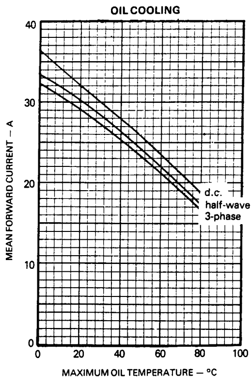
DERATING CURVES
