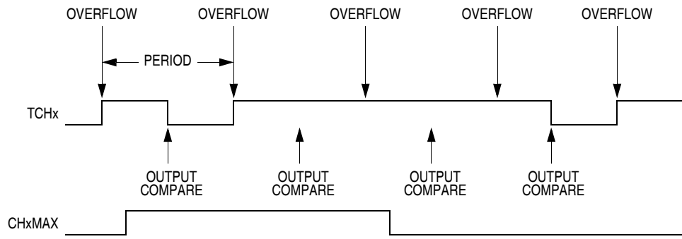
Figure 14-8. CHxMAX Latency
