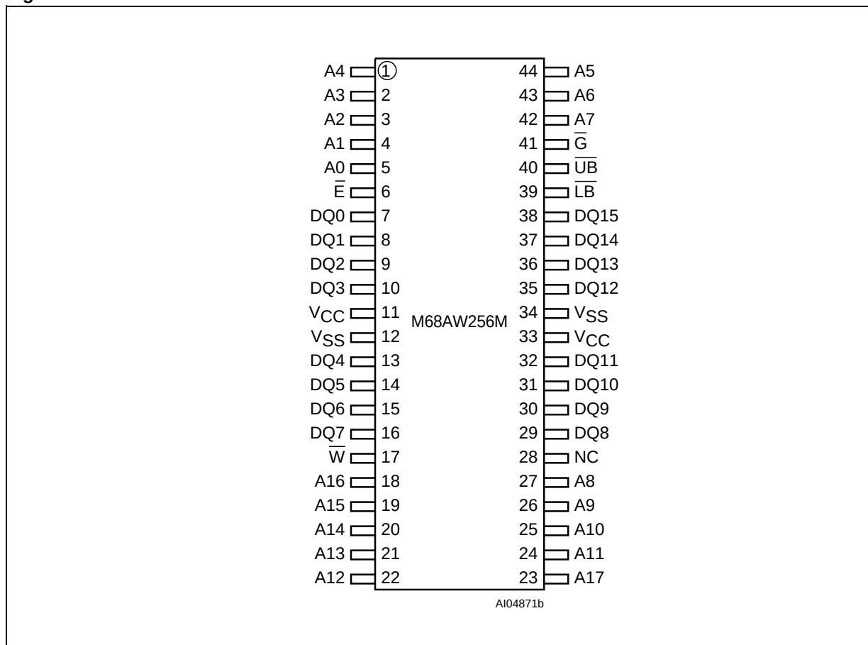
Figure 3. TSOP Connections
