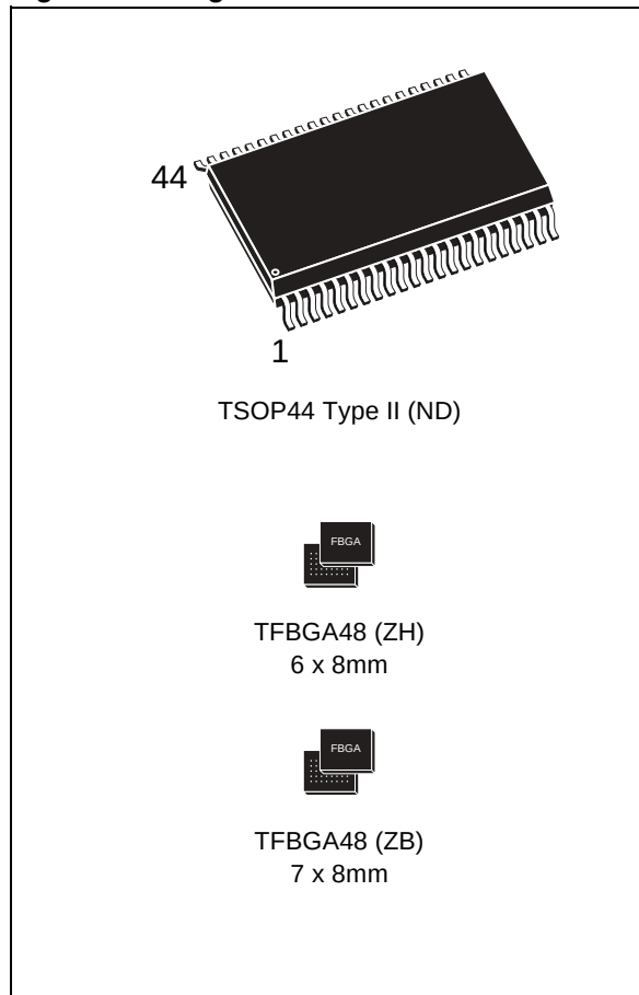
Figure 1. Packages
