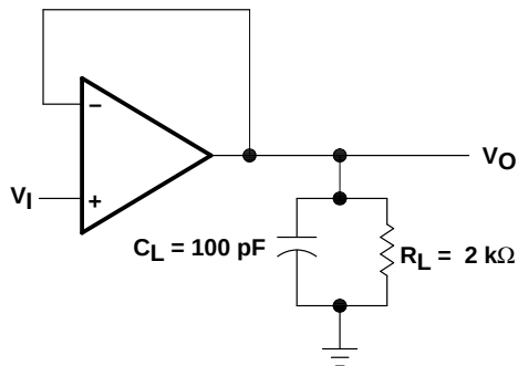
Figure 1. Unity-Gain Amplifier
