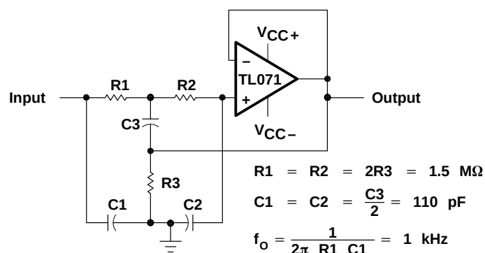
Figure 24. High-Q Notch Filter
