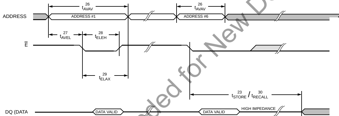
Figure 9. \overline{E} and \overline{G} Controlled Software STORE/RECALL Cycle [14]
