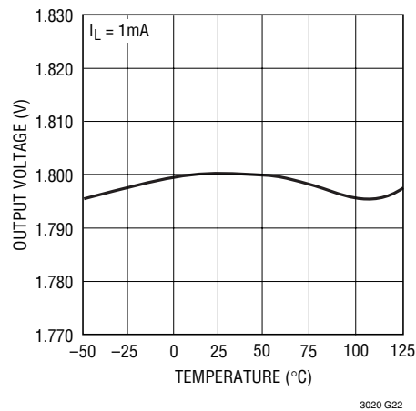
Output Voltage
