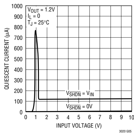
Quiescent Current
