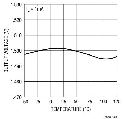
Output Voltage
