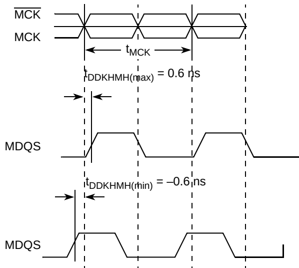
Figure 7. Timing Diagram for t_{\text{DDKMHM}}
