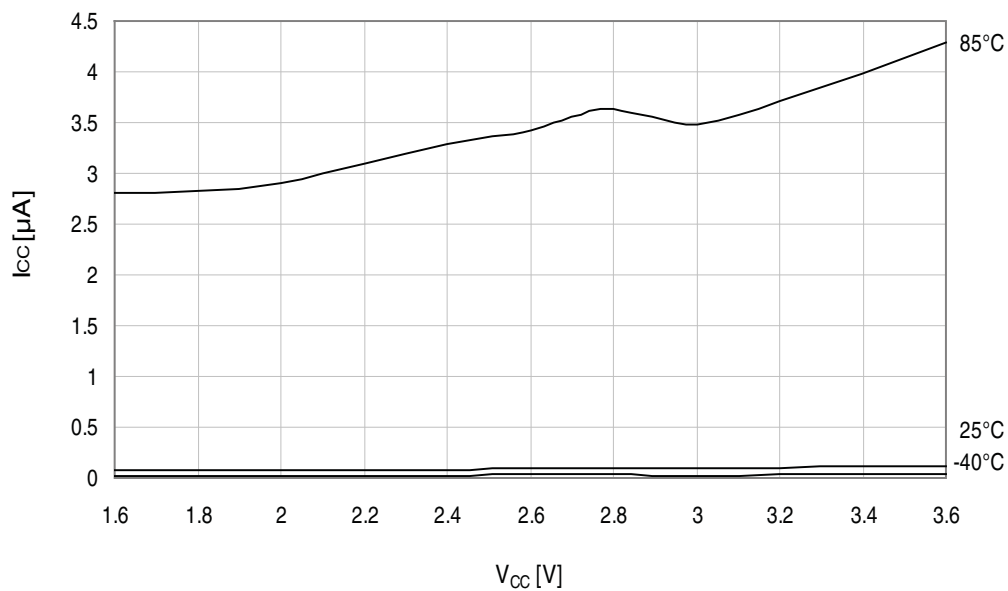
Figure 36-16. Power-down mode supply current vs. V_{CC} .
