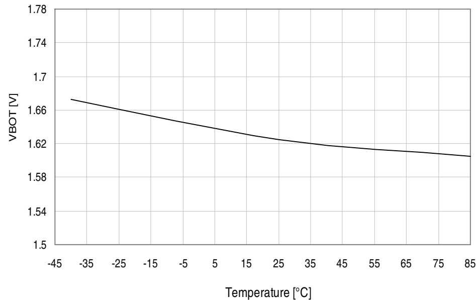
Figure 36-46.BOD thresholds vs. temperature.
