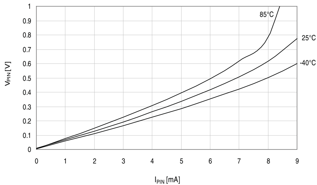
Figure 36-24. I/O pin output voltage vs. sink current.
