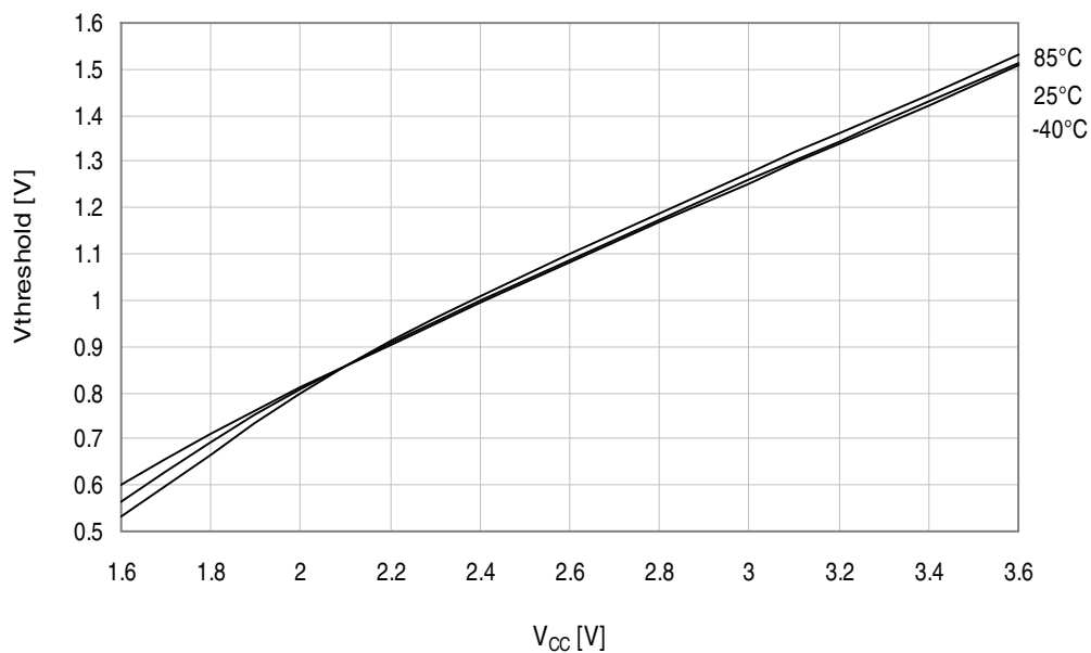
Figure 36-28. I/O pin input threshold voltage vs. V_{CC} .
