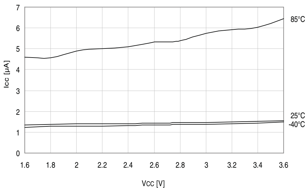
Figure 36-16. Power-down mode supply current vs. V_{CC} .
