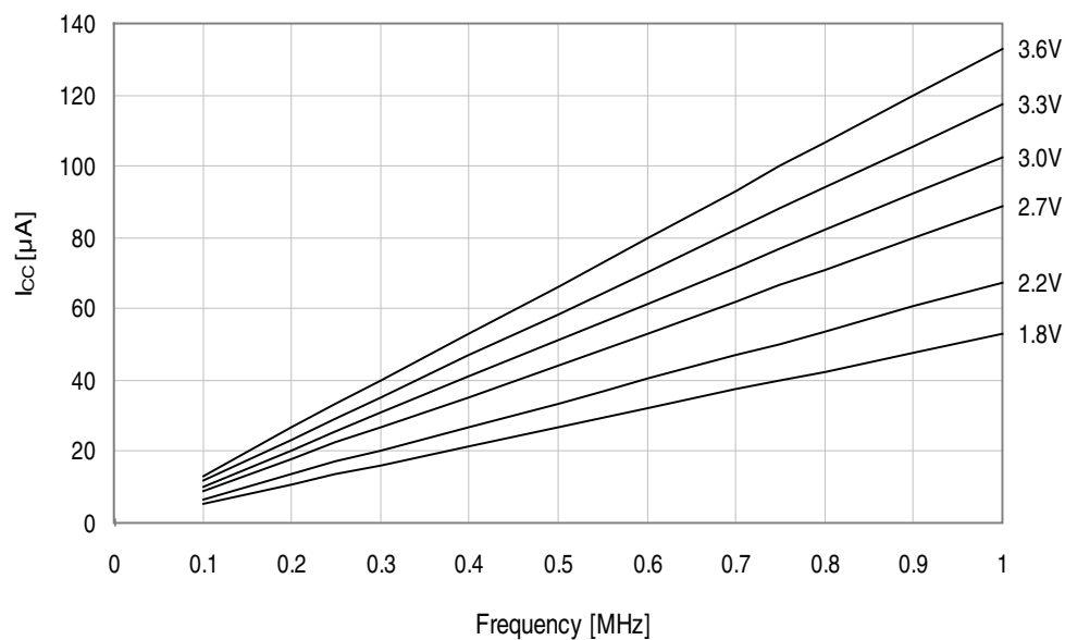
Figure 36-8. Idle mode supply current vs. frequency.
