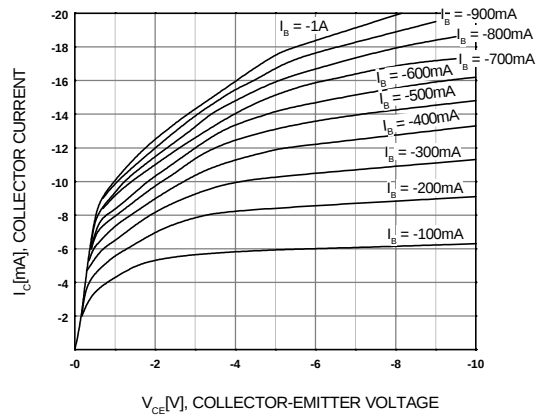
Figure 1. Static Characteristic
