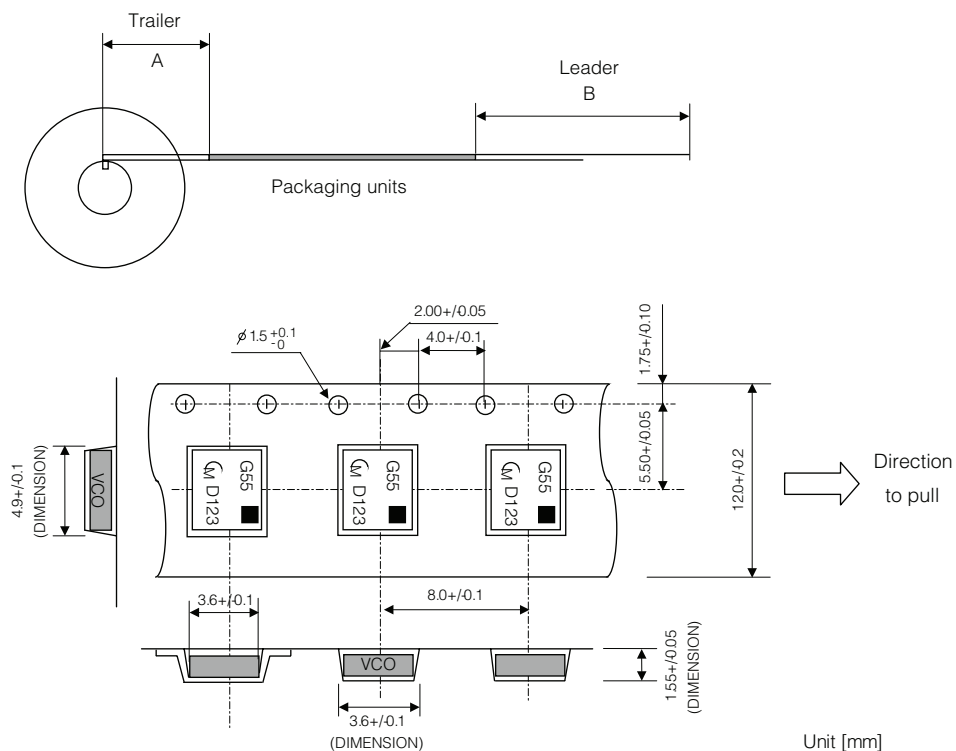
Figure 5-1: Tape Specification
