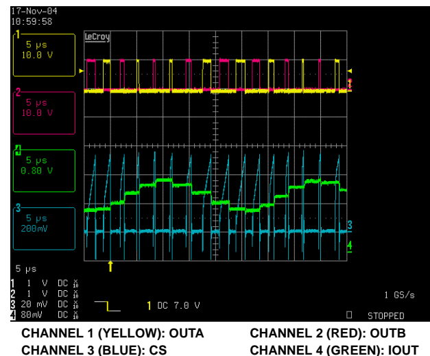
FIGURE 6. DYNAMIC BEHAVIOR OF CS vs IOUT
