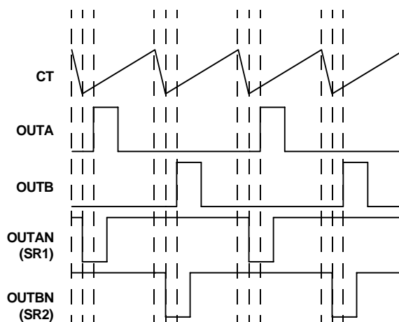
FIGURE 12. WAVEFORM TIMING WITH PWM OUTPUTS DELAYED, 0\text{V} < \text{VADJ} < 2.425\text{V}
