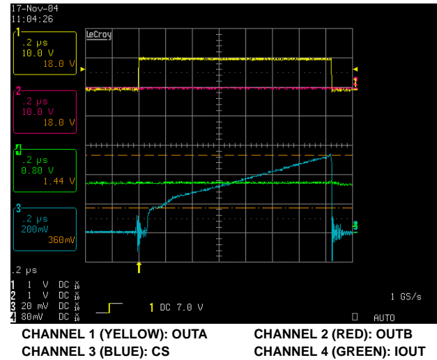
FIGURE 5. CS INPUT vs IOUT
