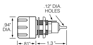
Watertight Product Dimensions
