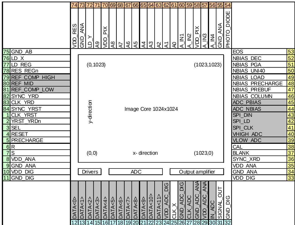
Figure 26. Pin Configuration
