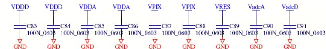
Figure 50. Reference Voltages End Circuit
