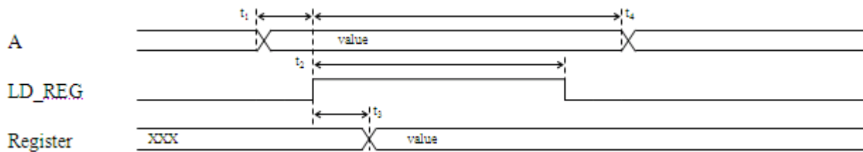
Figure 43. Mode Registers Upload Timing Diagram
