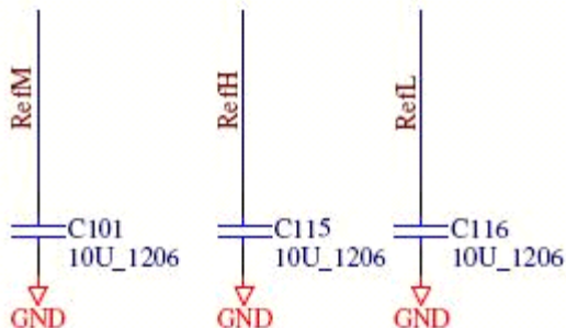
Figure 50. Reference Voltages End Circuit
