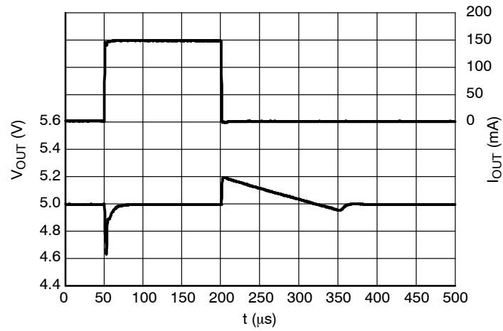
Figure 33. Load Transients, 5.0 V Version, I_{\text{OUT}} = 1 - 150 \text{ mA} , t_{\text{R}} = t_{\text{F}} = 0.5 \mu\text{s} , V_{\text{IN}} = 6.0 \text{ V}
