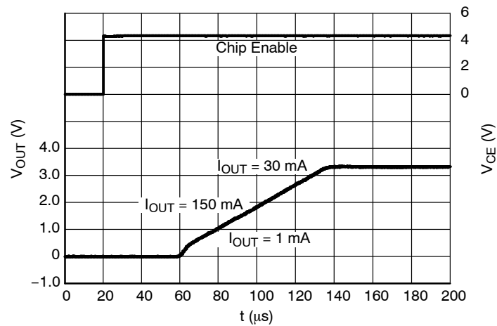
Figure 35. Start-up, 3.3 V Version, V_{\text{IN}} = 4.3 \text{ V}
