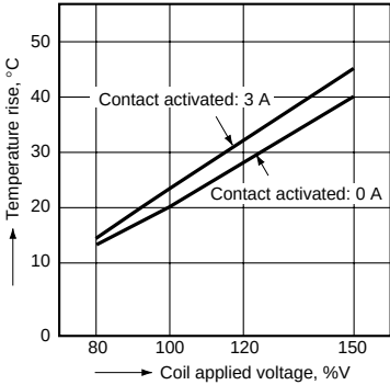
1.-(2) Coil temperature rise (DC PC board type)
