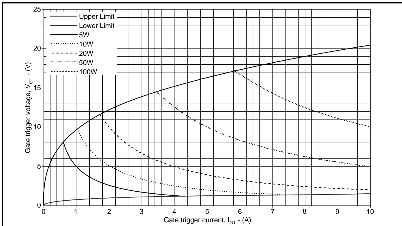
Fig.8 Gate characteristics
