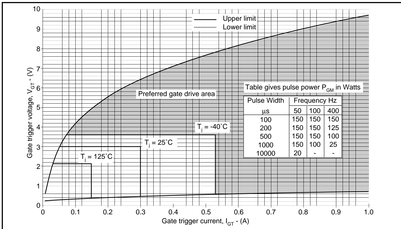
Fig.7 Gate characteristics
