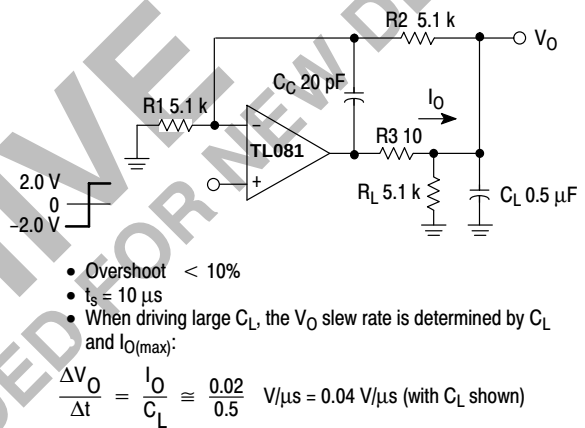
Figure 17. Isolating Large Capacitive Loads
