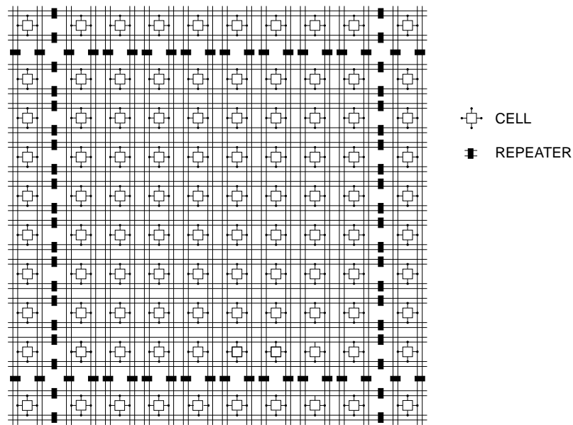
Figure 3. Cell-to-Cell and Bus-to-Bus Connections
