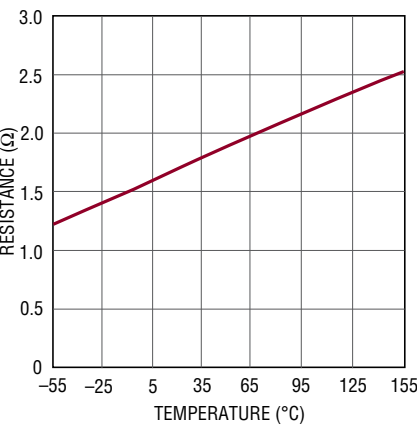
V AUX Drop-Out Resistance vs Temperature
