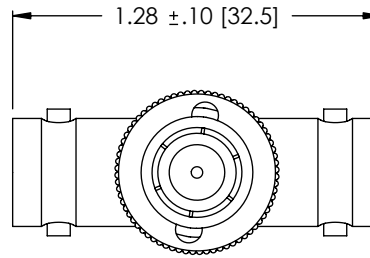
BNC PLUG
