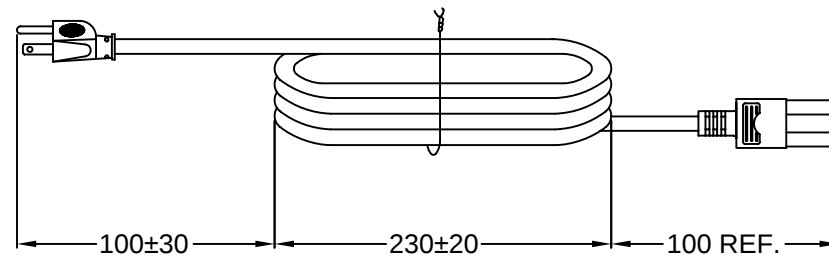
HANKING DETAIL
