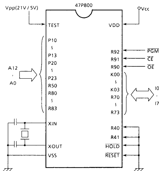
Figure 1-3. Setting for PROM mode
