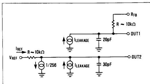
Figure 2. AD7524/MAX7624 DAC Equivalent Circuit—All Digital Inputs LOW
