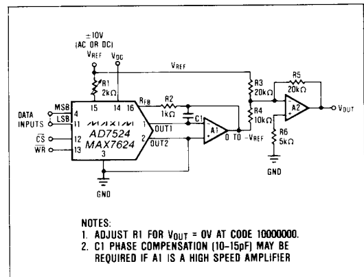
Figure 4. Bipolar (4-Quadrant) Operation
