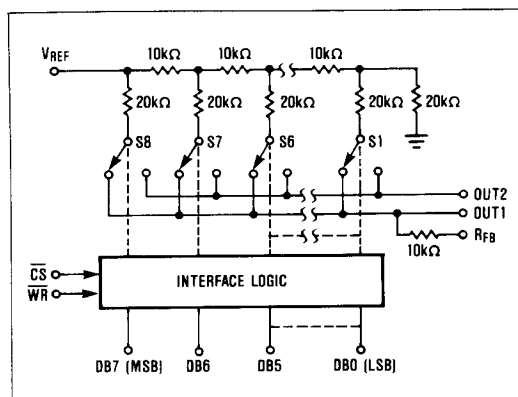
Figure 1. AD7524/MAX7624 Functional Diagram
