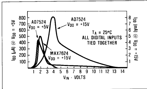
Figure 3. Typical Supply Current, I_{DD} vs. Logic Input Voltage V_{IN} , for V_{DD} = +5V and +15V
