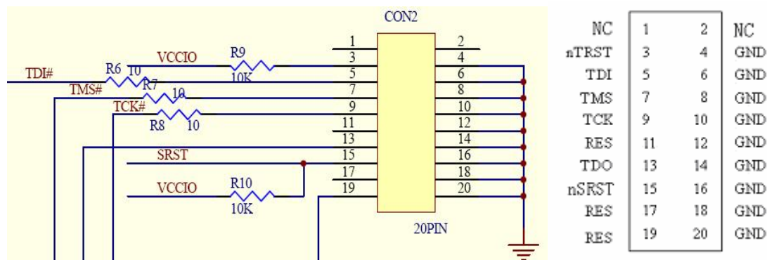
Emlink JTAG Signal 20pins
