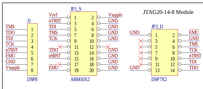
Emlink JTAG Signal Definition
