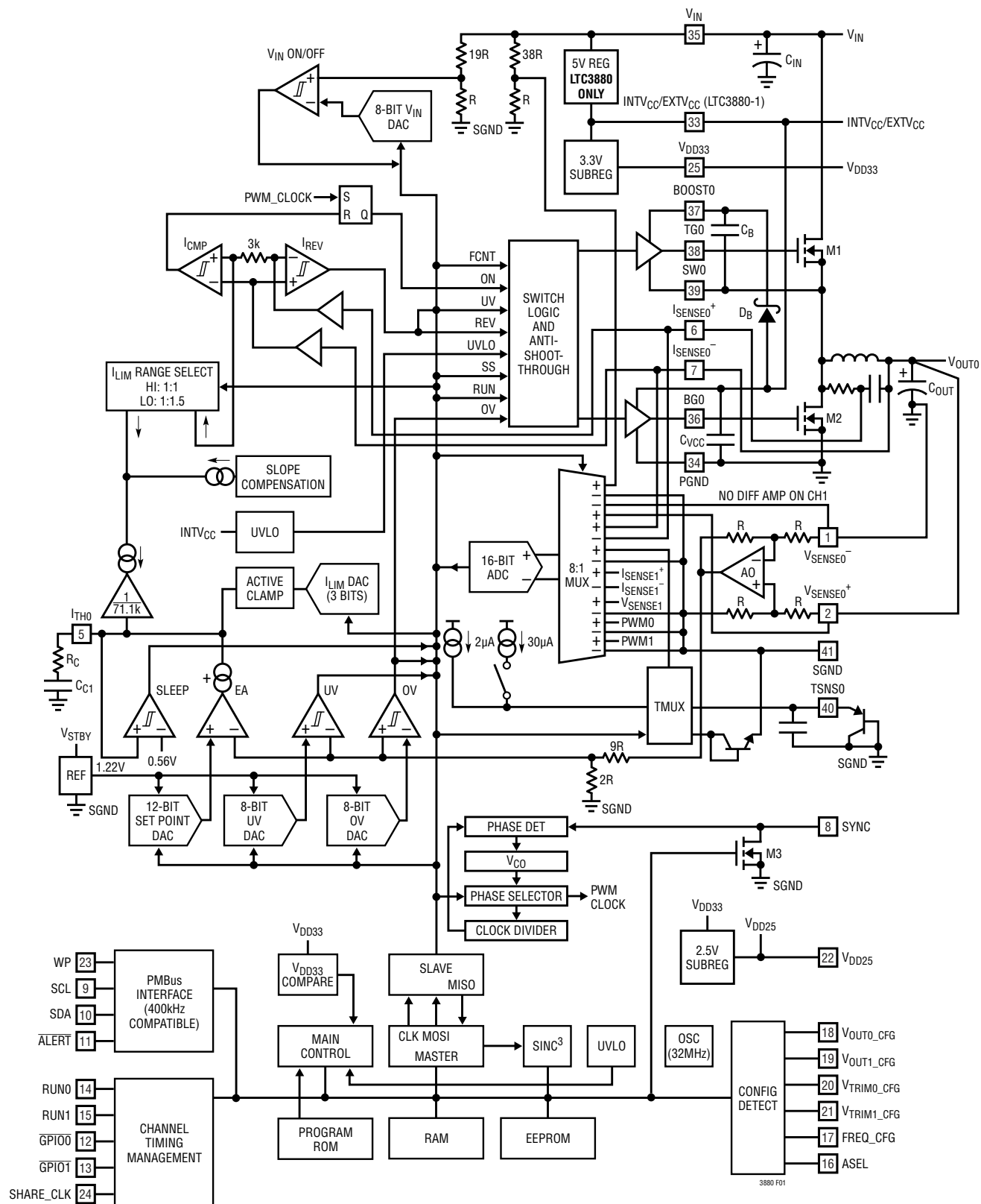
Figure 1. Block Diagram
