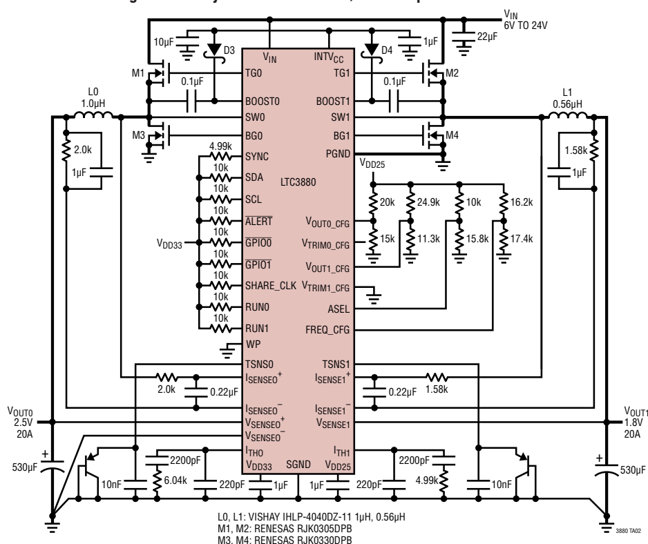
High Efficiency Dual 425kHz 2.5V/1.8V Step-Down Converter
