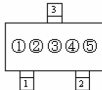
SOT-23-3L (TOP-VIEW)
