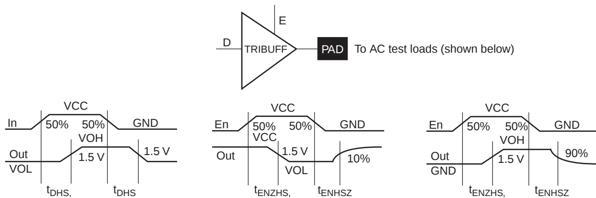
Figure 2-11 • Output Buffers
