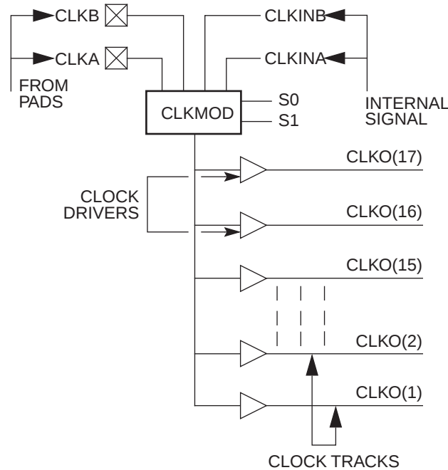
Figure 2-6 • Clock Networks
