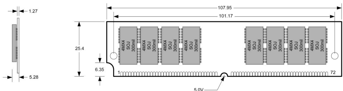
Figure1: mechanical dimensions
