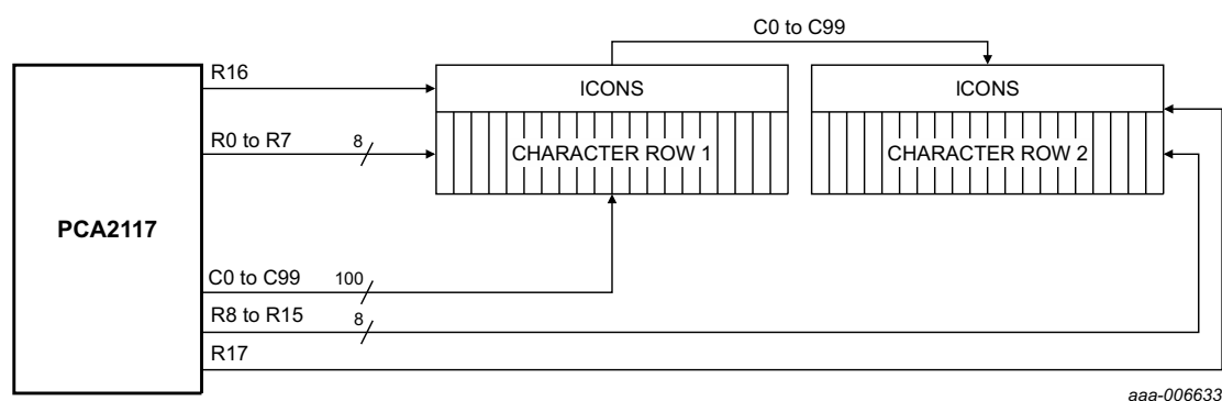
Fig 15. Connecting PCA2117 with a 1 × 40 character LCD
