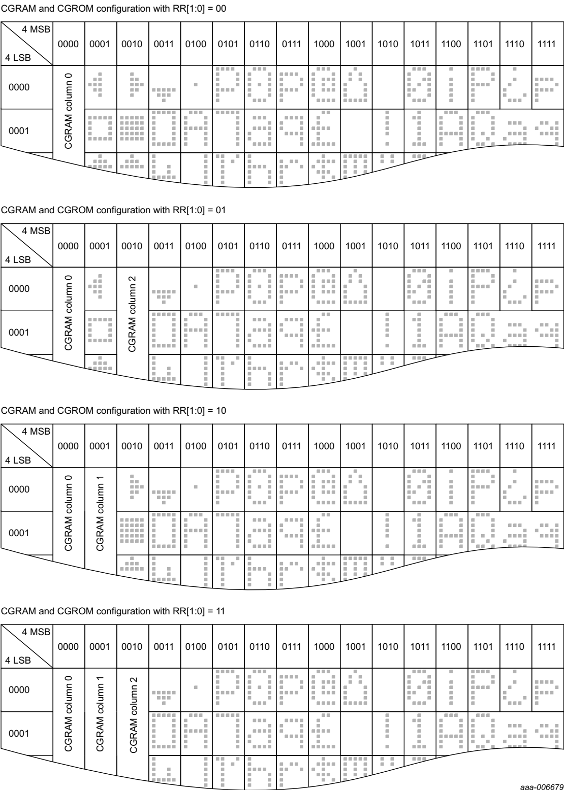
Fig 36. Configuration of CGROM and CGRAM with RR[1:0]
