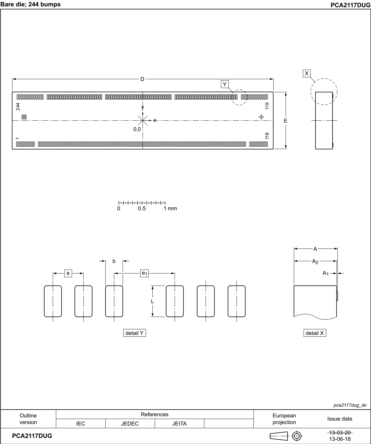
Fig 64. Bare die outline of PCA2117DUGx
