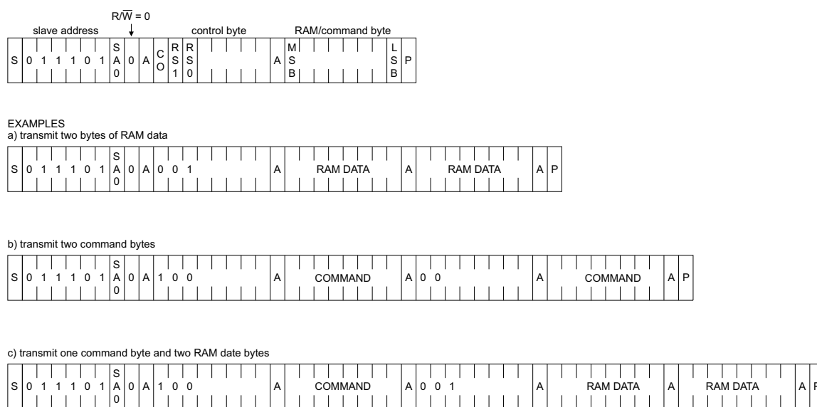
Fig 50. I 2 C-bus protocol write mode
