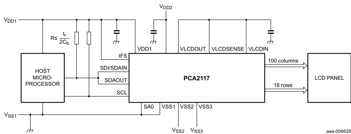
V DD1 and V DD2 from 2.5 V to 5.5 V. Values for t r and C b , see Table 48 . V DD1 and V DD2 can be connected to the same power supply. V SS1 to V SS3 can be connected to the same ground supply.
