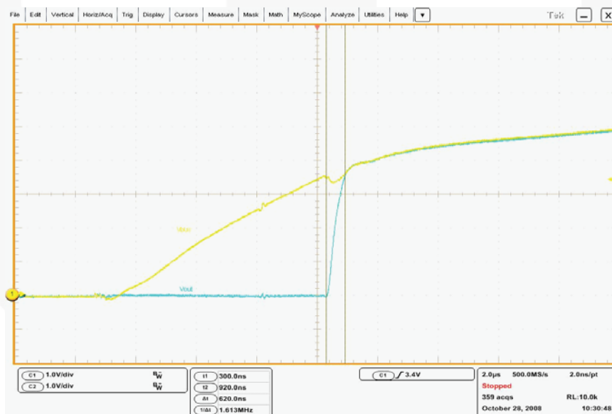
Figure 7. Turn-On Time
