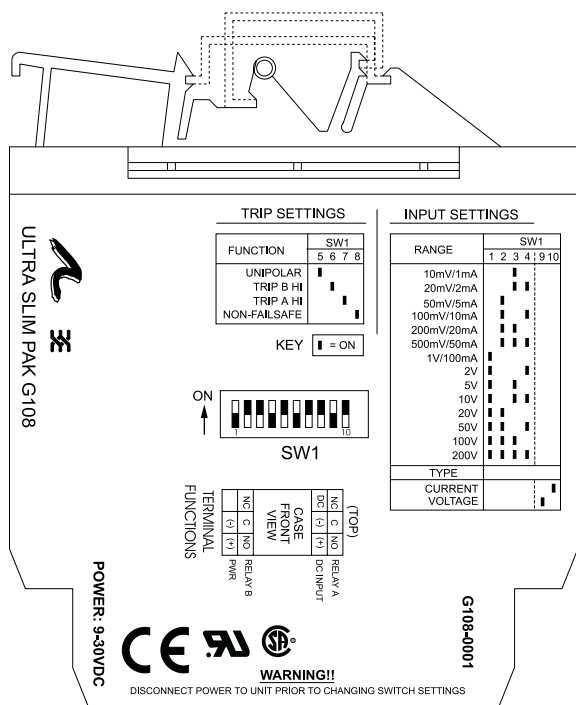
Figure 5: G108 Factory Cal; 0-20mA, A-HI/B-LO, Non-Failsafe
