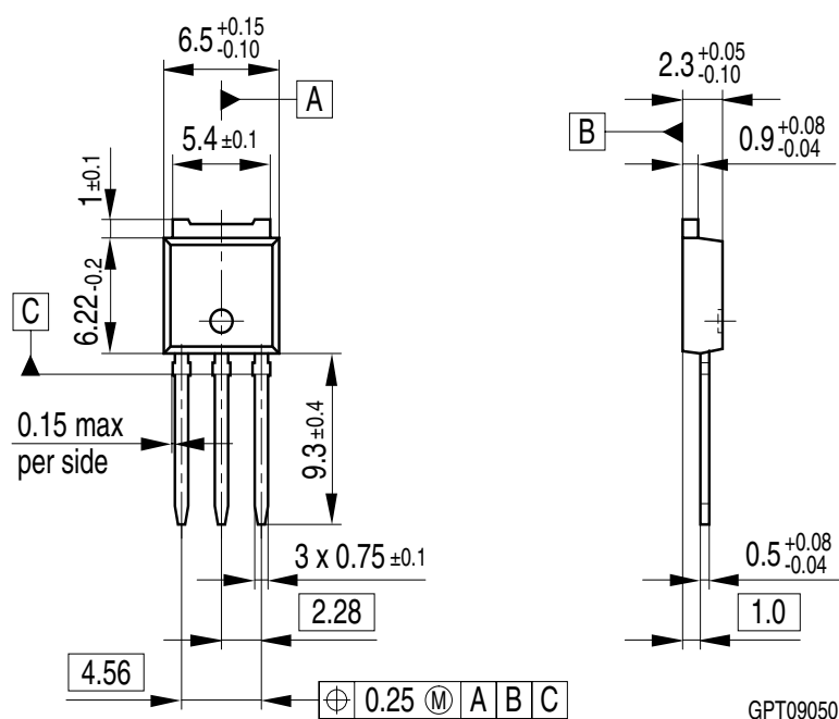
P-TO-251-3-1 (I-PAK)
