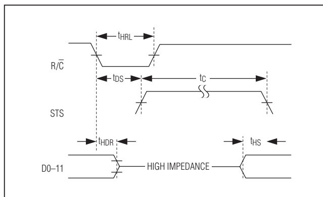
Figure 6. Low Pulse for \overline{R/\overline{C}} in Stand-Alone Mode
