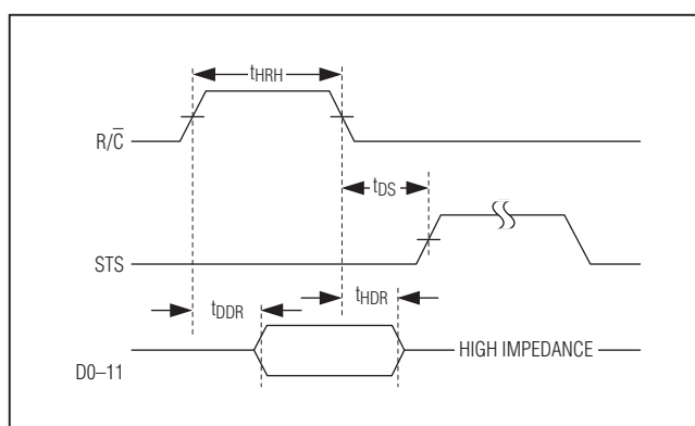
Figure 7. High Pulse for \overline{R/\overline{C}} in Stand-Alone Mode
