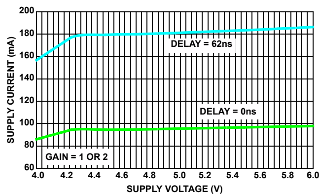
FIGURE 25. ISL59920 I_{SUPPLY+} vs V_{SUPPLY+}
