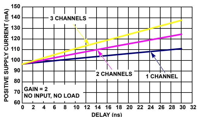
FIGURE 24. ISL59923 POSITIVE SUPPLY CURRENT ( V_{SP} ) vs DELAY TIME
