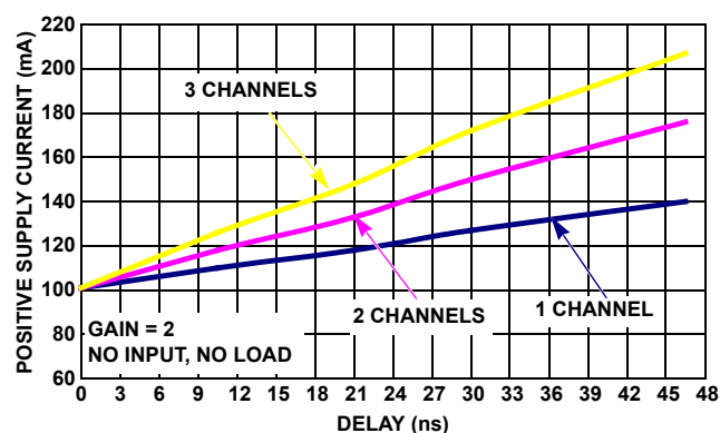
FIGURE 22. ISL59921 POSITIVE SUPPLY CURRENT ( V_{SP} ) vs DELAY TIME
