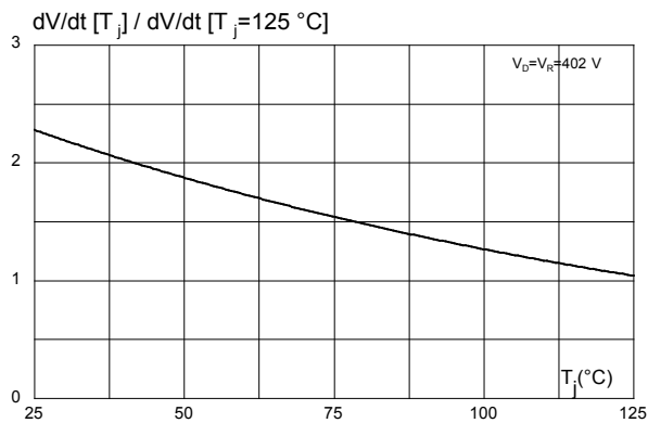
Figure 9. Relative variation of static dV/dt immunity versus junction temperature
