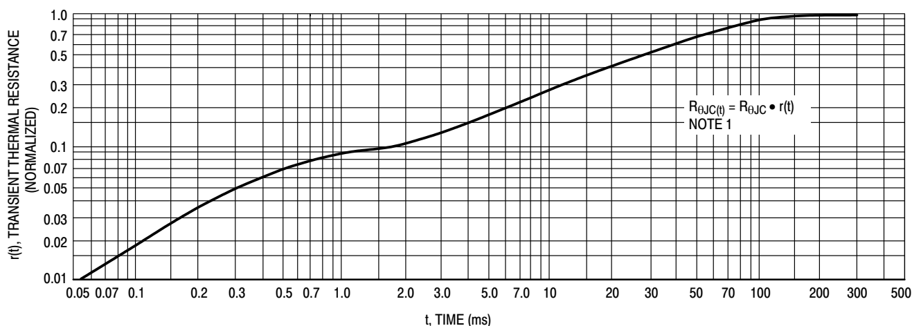
Figure 6. Thermal Response
