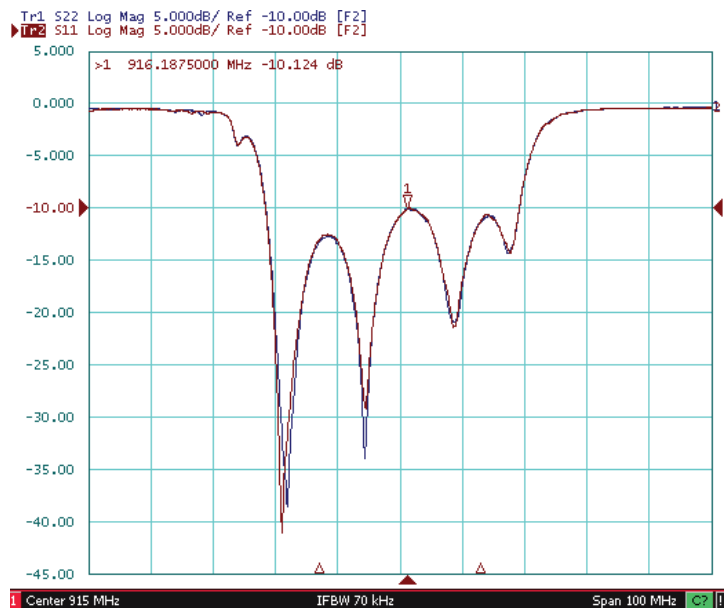
Return Loss
