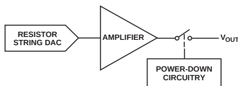
Figure 9. Output Stage During Power-Down
