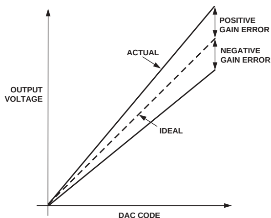
Figure 4. Gain Error
