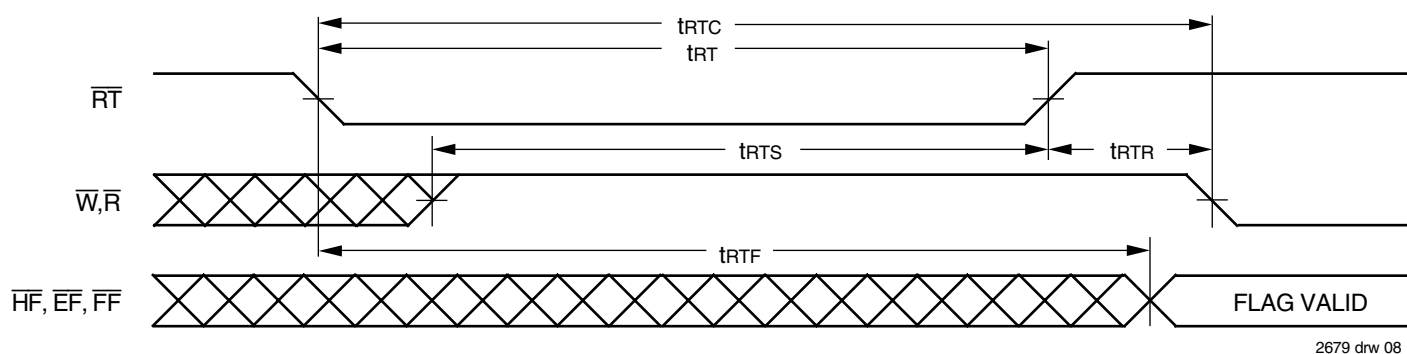
Figure 6. Retransmit
