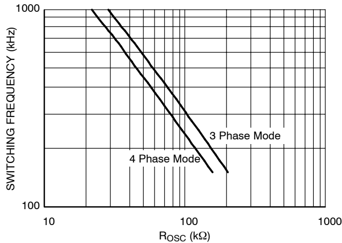
Figure 7. Oscillator Frequency versus Total R_{osc} Value
