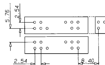
PCB FOOTPRINT WITHOUT STRAIN RELIEF
