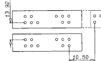
PCB FOOTPRINT WITH STRAIN RELIEF
