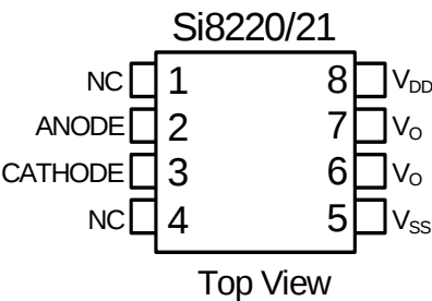
Figure 17. Pin Configuration
