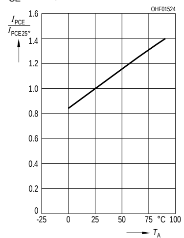
Photocurrent I_{\text{PCE}} = f(T_A) ,
