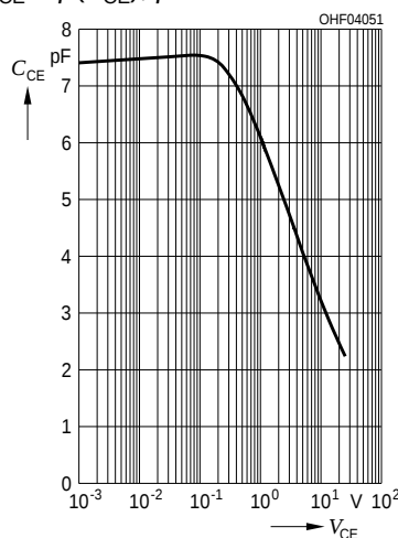
Capacitance
