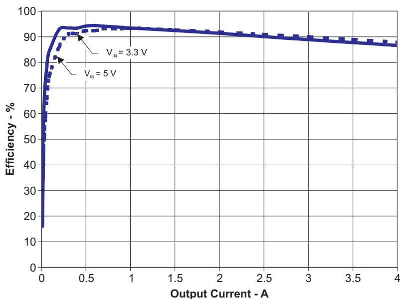
Figure 1. TPS54478EVM-037 Efficiency
