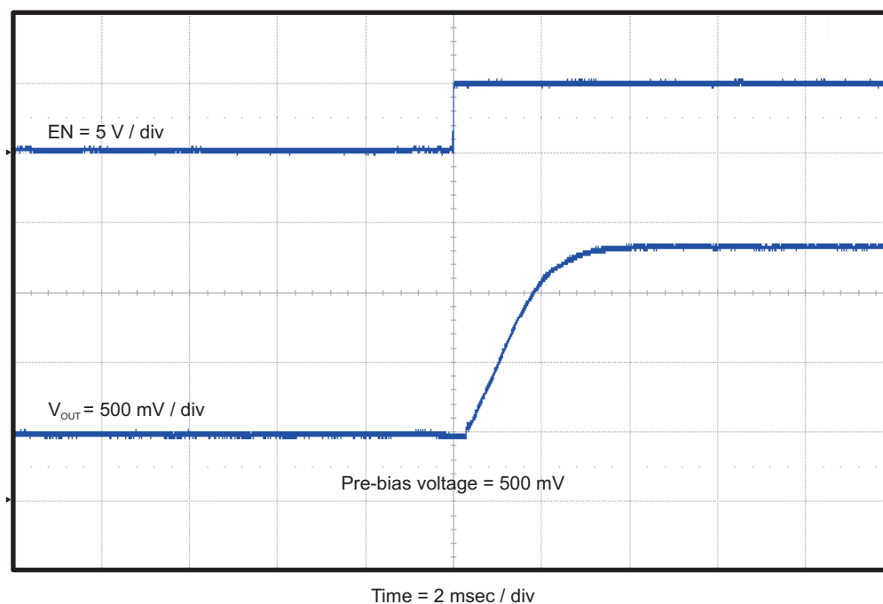
Figure 11. TPS54478EVM-037 Start-up into Pre-bias
