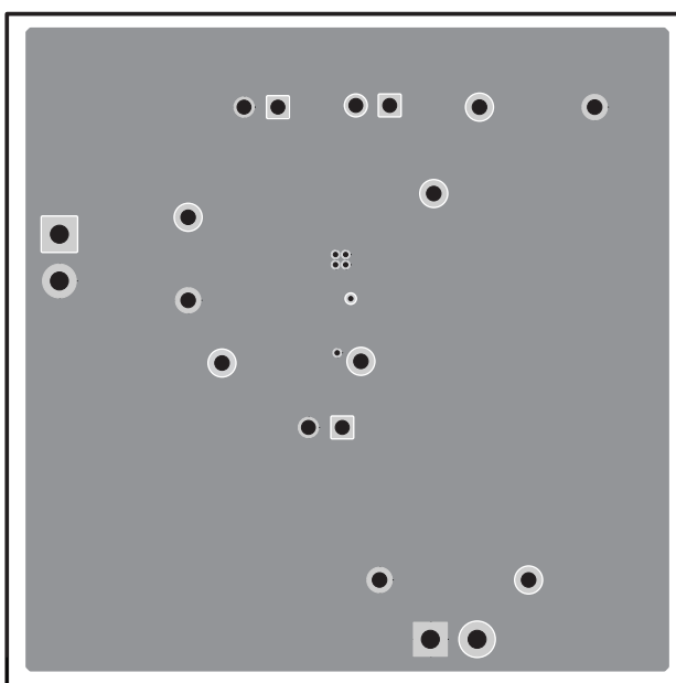
Figure 18. TPS54478EVM-037 Layout 2
