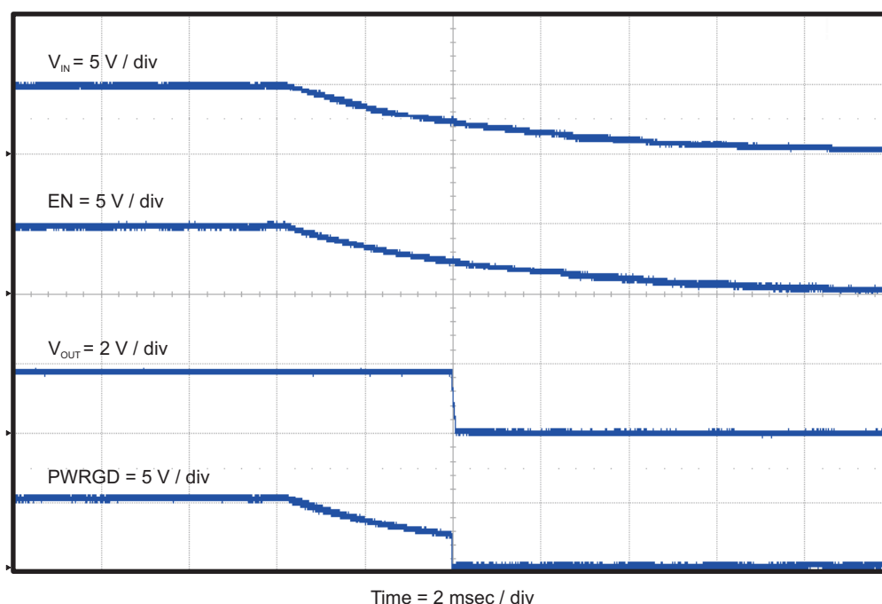
Figure 12. TPS54478EVM-037 Shut-down Relative to V_{IN}
